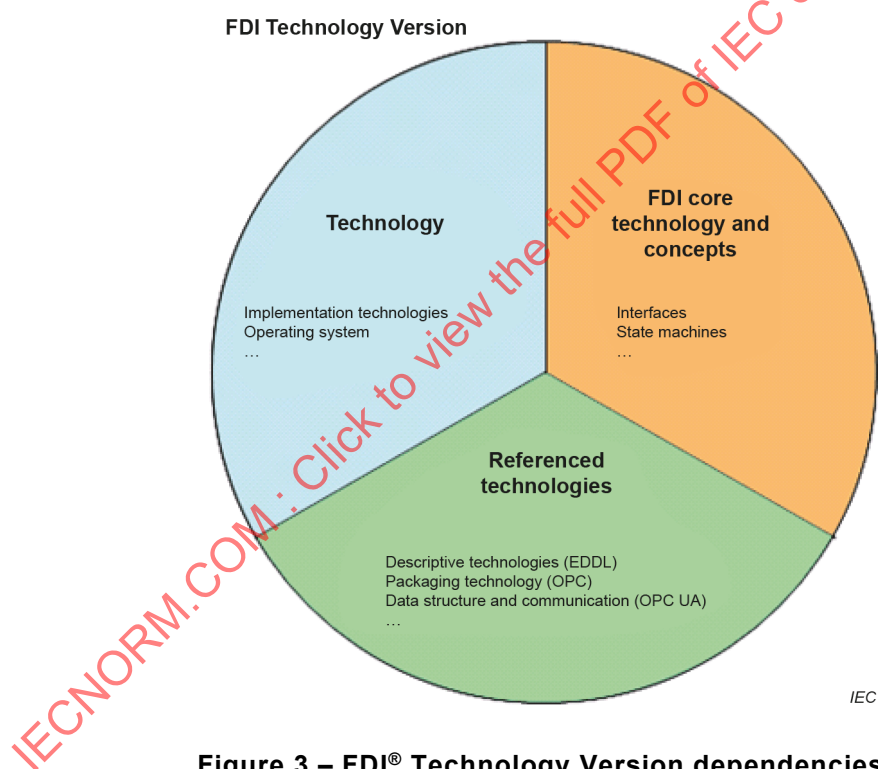
Figure 3 – FDI® Technology Version dependencies
