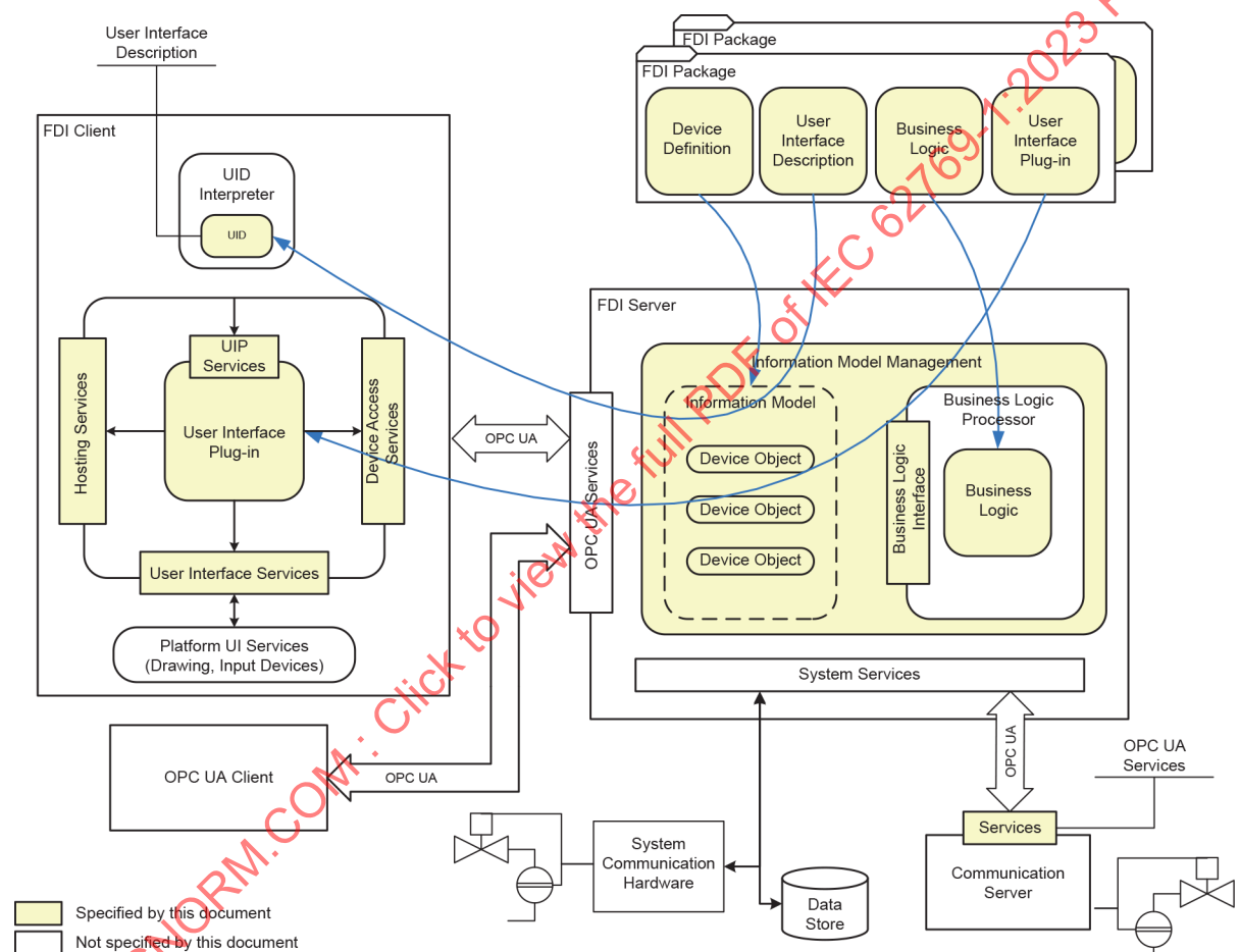
Figure 1 – FDI® architecture diagram
