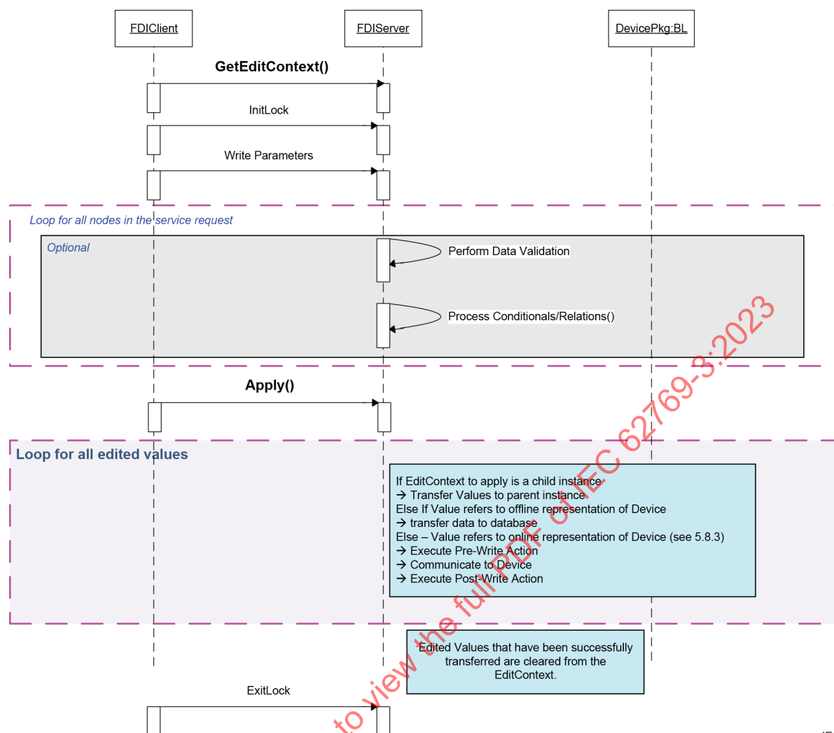
Figure 11 – Write with EditContext
