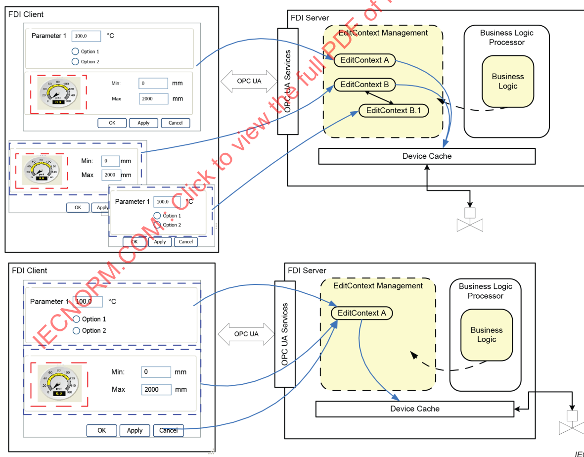
Figure 3 – EditContext models
