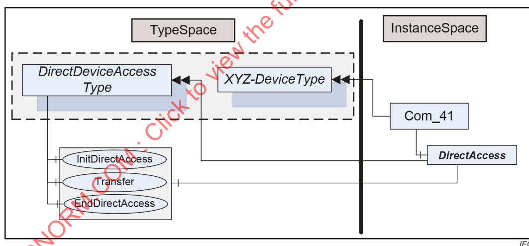
Figure 19 – DirectDeviceAccess instance
