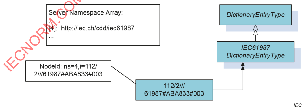
Figure 11 – Example of concrete DictionaryEntryType and Object
