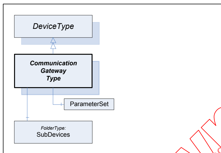
Figure 13 – CommunicationGatewayType
