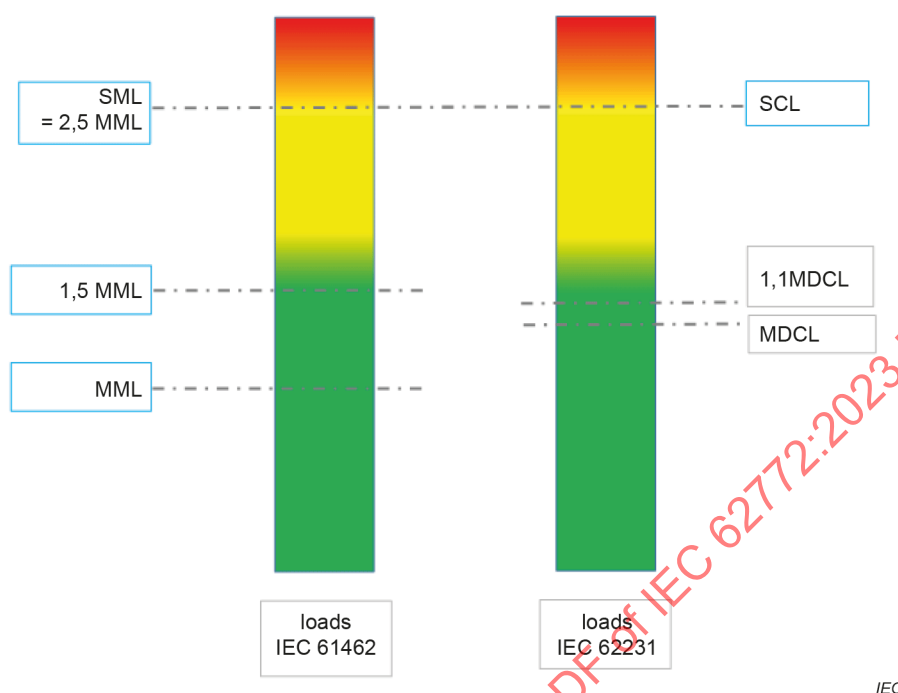
Figure B.3 – Comparison of definitions IEC 61462 vs. IEC 62231
