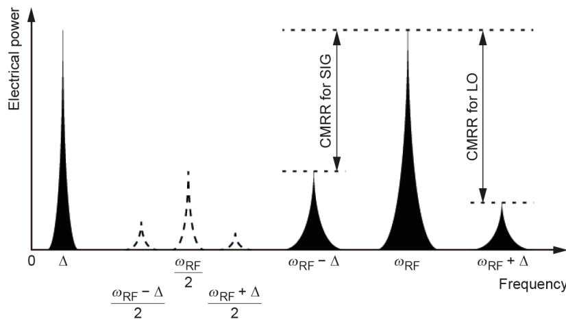
Figure 3 – Schematic illustration of the electric power spectra of the signal measured by the electrical spectrum analyser
