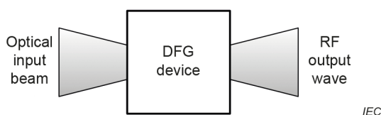
Figure 2 – DFG device
