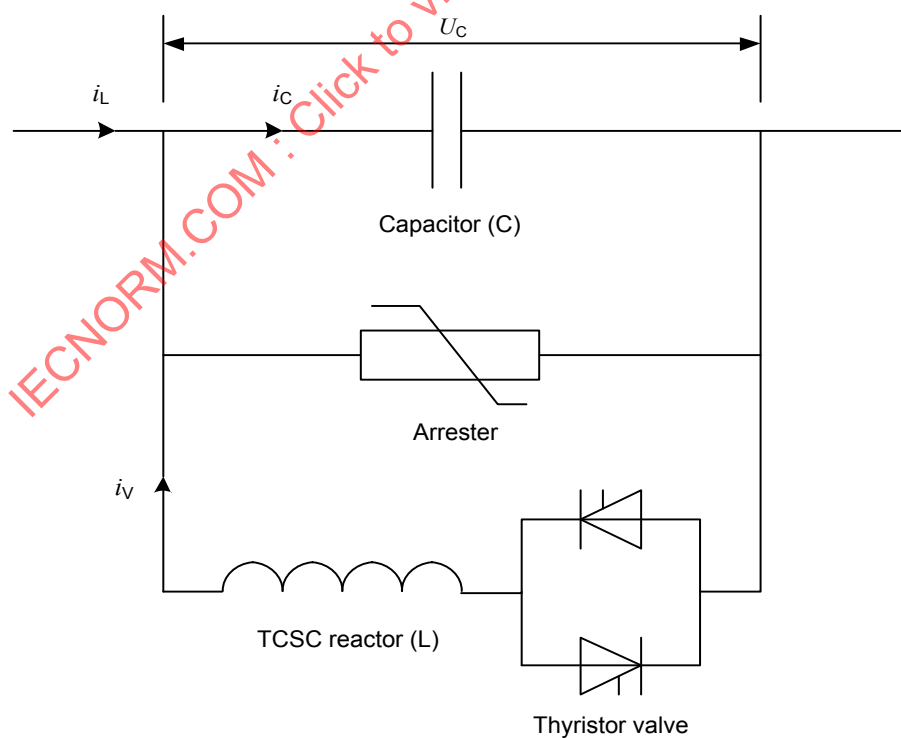
Figure 2 – TCSC subsegment
