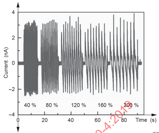
Figure C.2 – The output current measurement for different types of stretching
