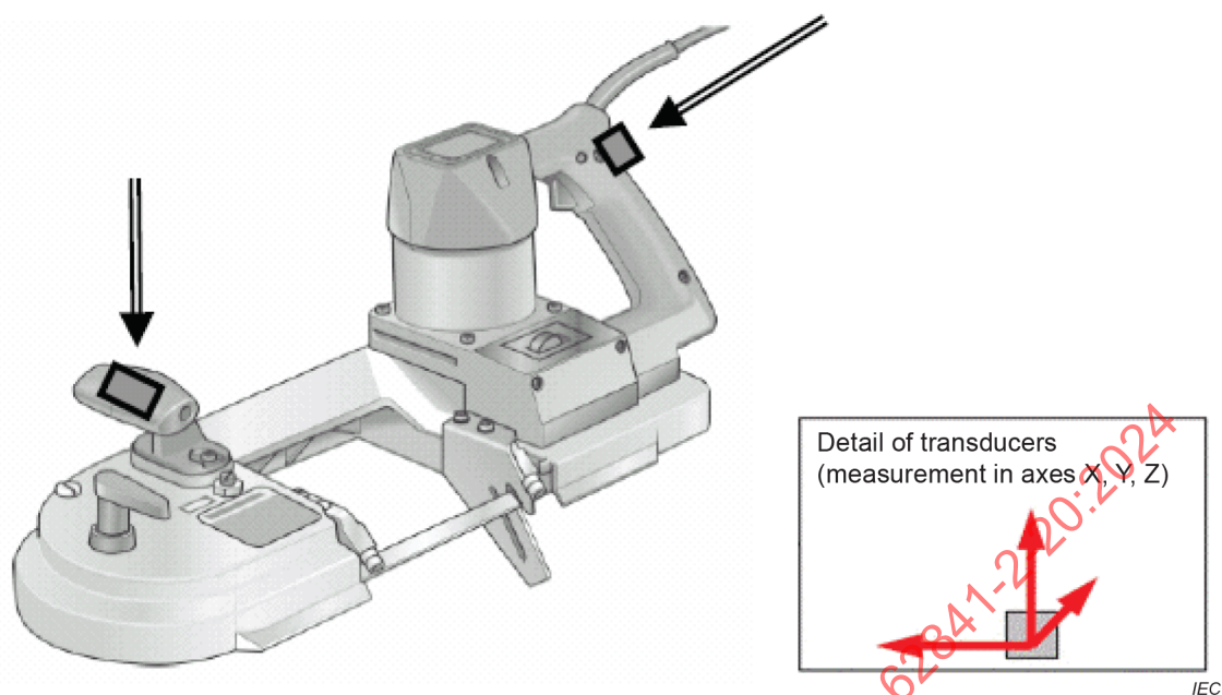
Figure I.101 – Positions of transducers for band saws
