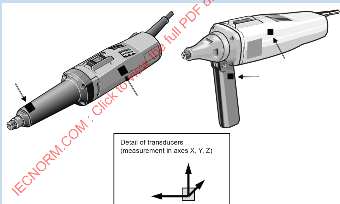
Figure I.101 – Positions of transducers for die grinders
