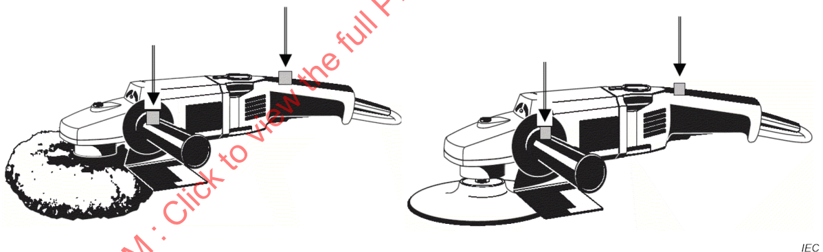
Figure I.103 – Positions of transducers for disc-type polishers and disc-type sanders
