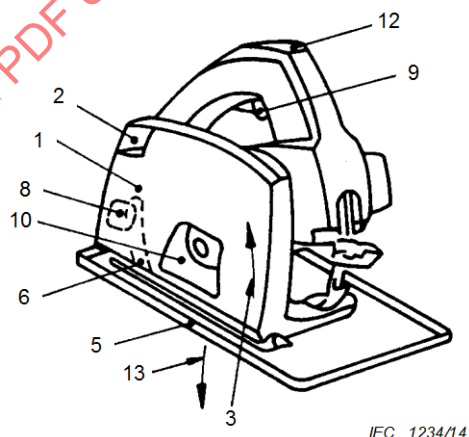
Figure 104 – Scie plongeante
