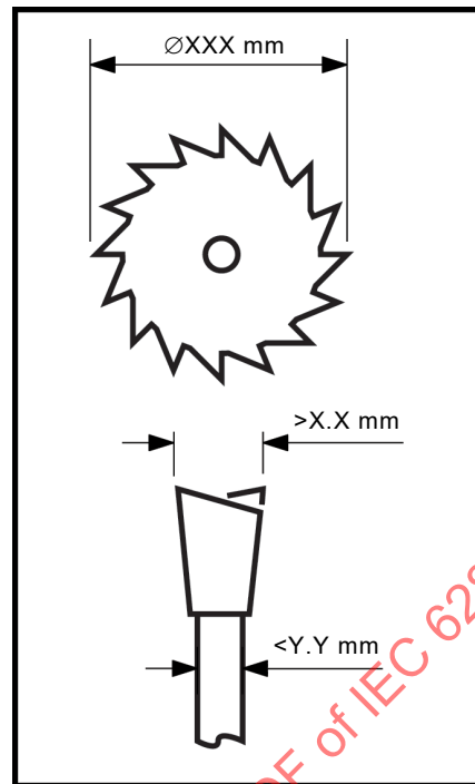
Figure 101 – Marking of the riving knife
