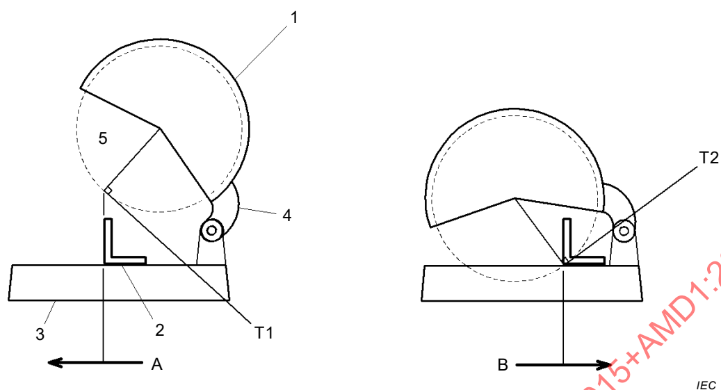
a) Cutting unit in rest position and in fully down position
