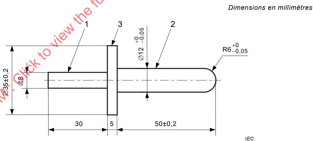
Figure 103 – Protectors de disque
