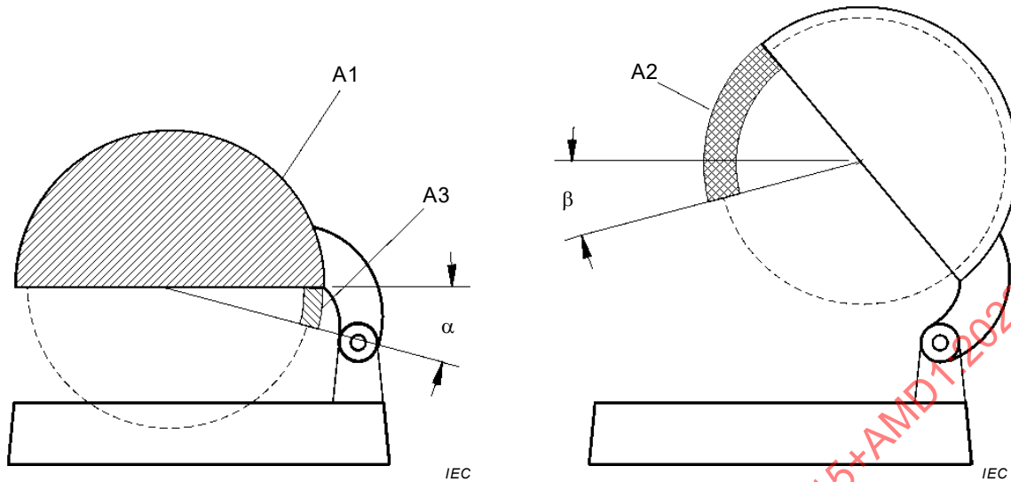
a) Cutting unit in fully down position
