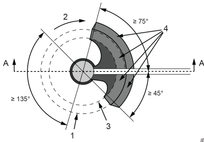
a) Plan view for lawn trimmers having cutting element energy \leq 10 J
