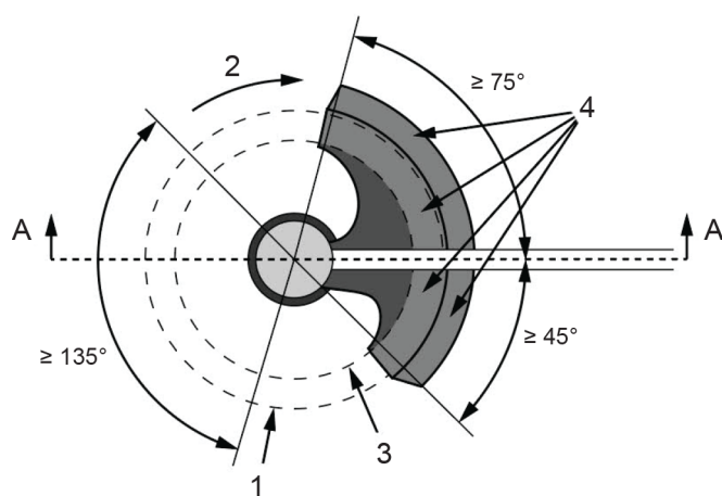
a) Plan view for lawn trimmers having cutting element energy \leq 10 J
