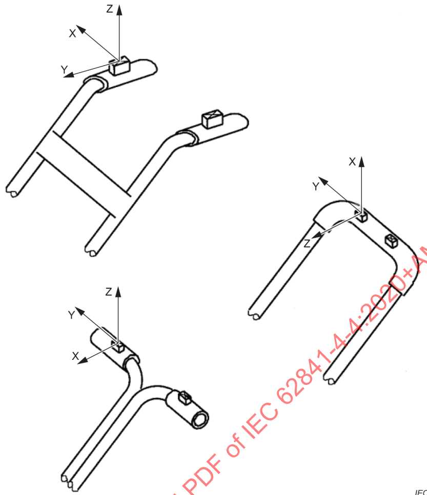
Figure I.103 – Examples of positions of transducers (walk-behind machines)
