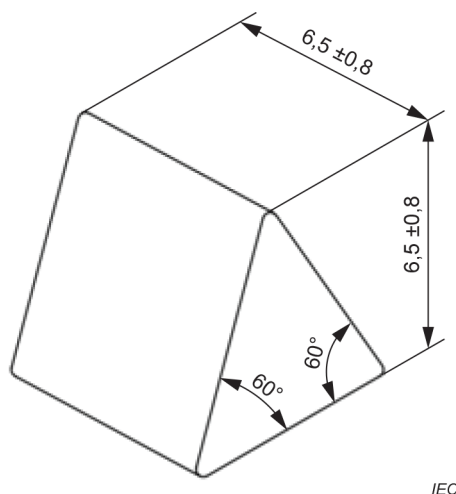
Figure 111 – Test piece
