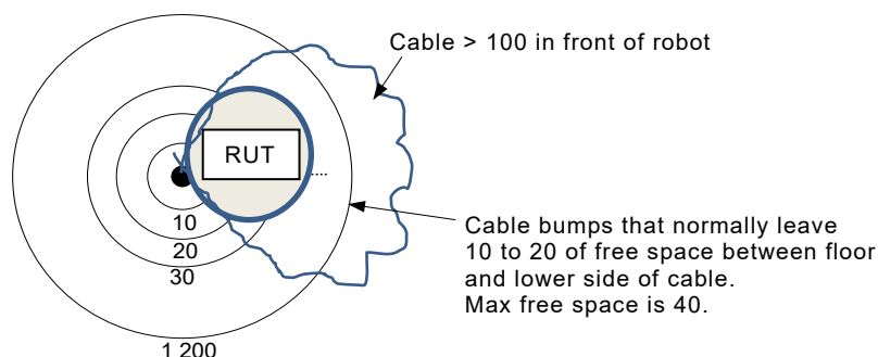
Figure 10 – Floor circle marks schematic diagram with robot
