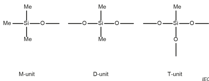
Figure A.1 – Representation of the molecular structure of M-, D-, and T-units in polydimethylsiloxanes (PDMS)
