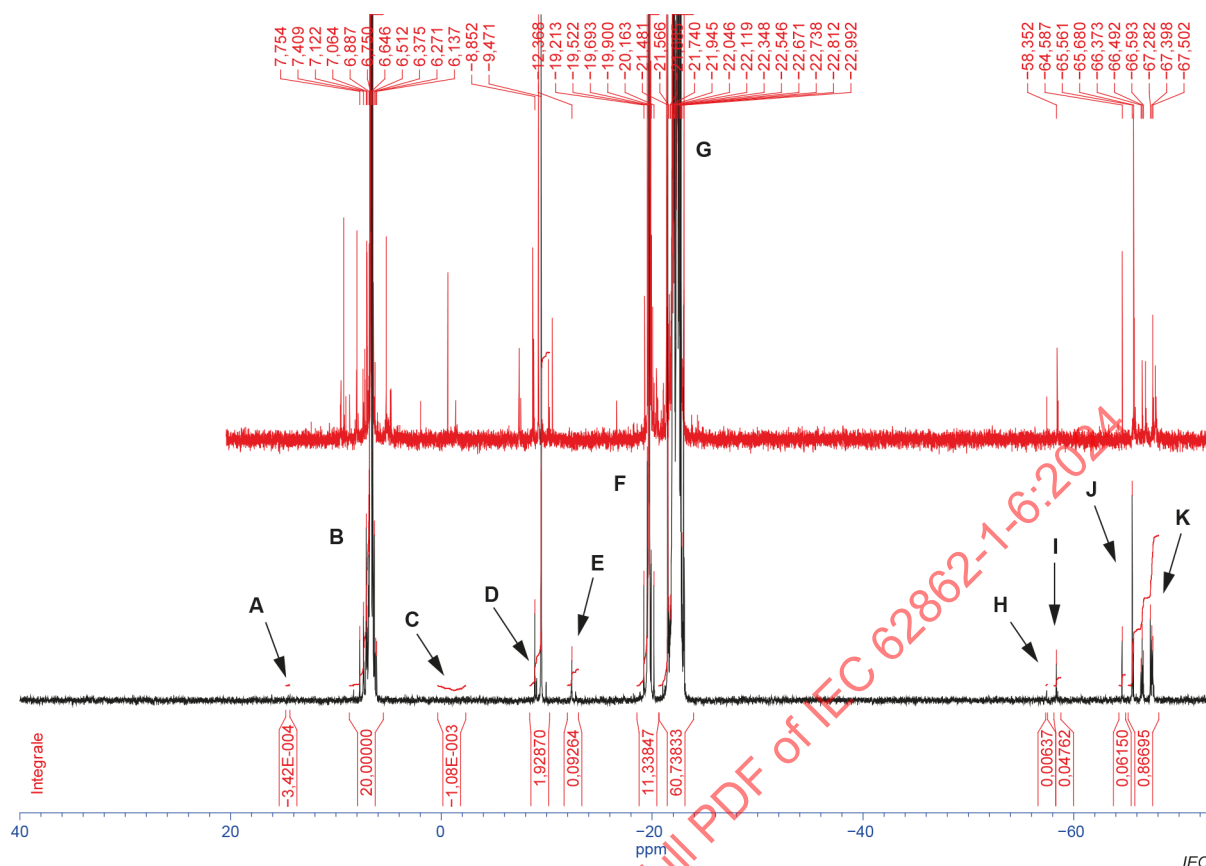
Figure A.5 – Representation of a ^{29}\text{Si} NMR spectrum indicating the different shift regions
