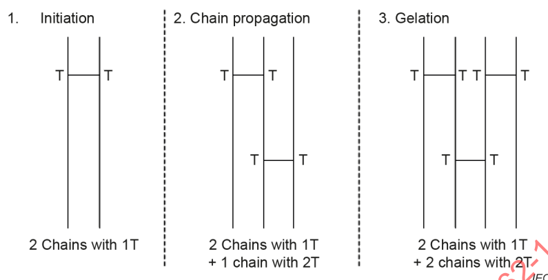
Figure A.4 – Theoretical model for describing the long-term increase in viscosity of polydimethylsiloxane-based fluids by thermal aging
