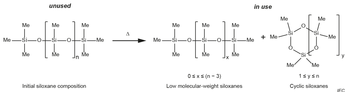
Figure A.2 – Representation of the molecular structure of polydimethylsiloxanes (PDMS, left) and the thermally induced equilibration reaction of linear polydimethylsiloxanes
