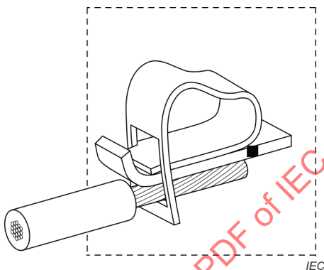
b) Screwless-type terminal with direct pressure
