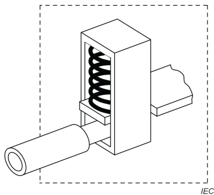
a) Screwless-type terminal with indirect pressure
