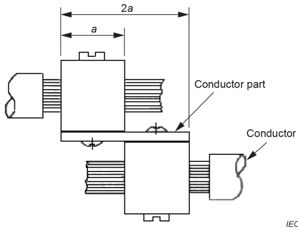
Figure 3 – Test specimen example 2
