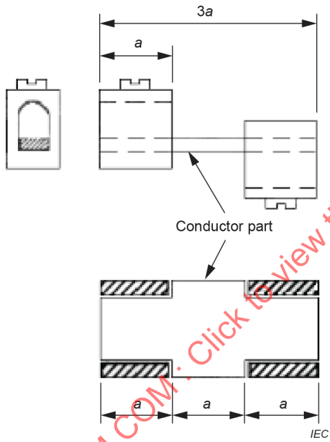
Figure 5 – Test specimen example 4
