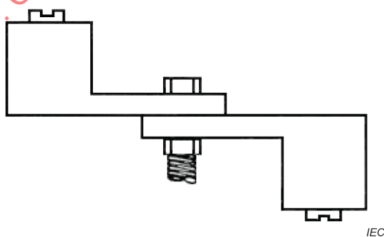
Figure 2 – Test specimen example 1
