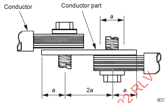
Figure 4 – Test specimen example 3
