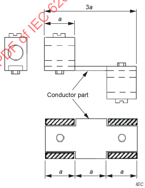
Figure 6 – Test specimen example 5
