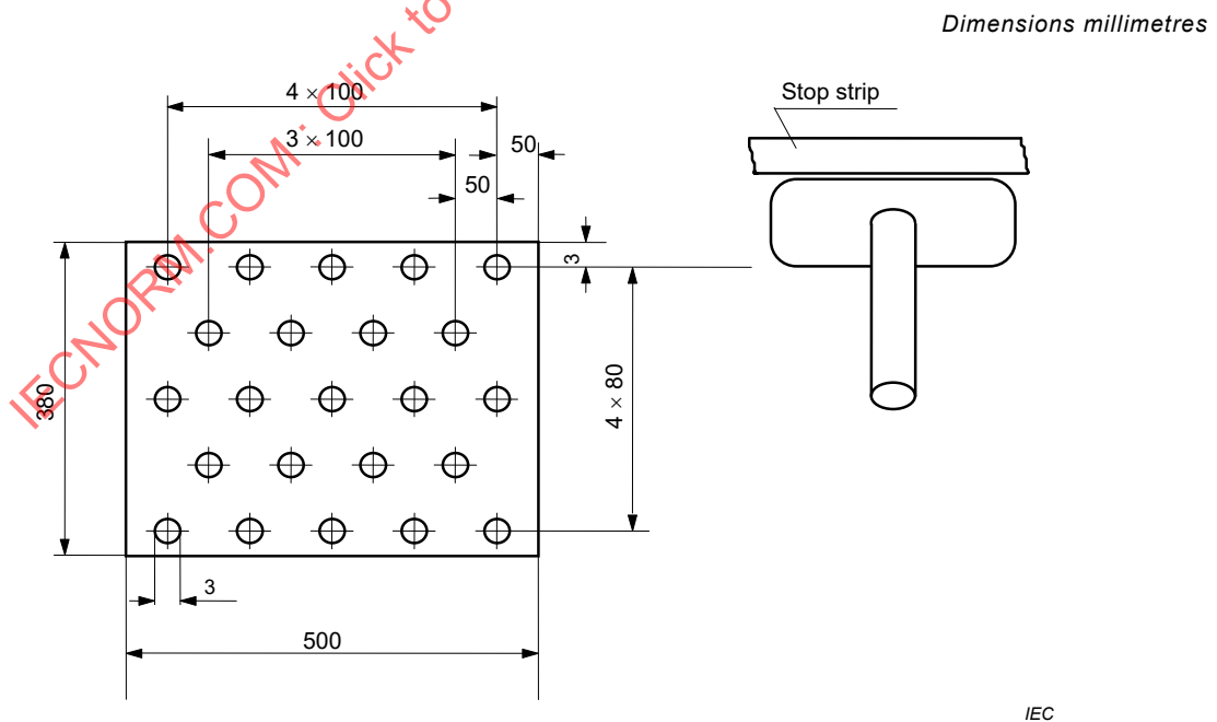
Figure 6 – Stencil for distribution of fibres on upholstery
