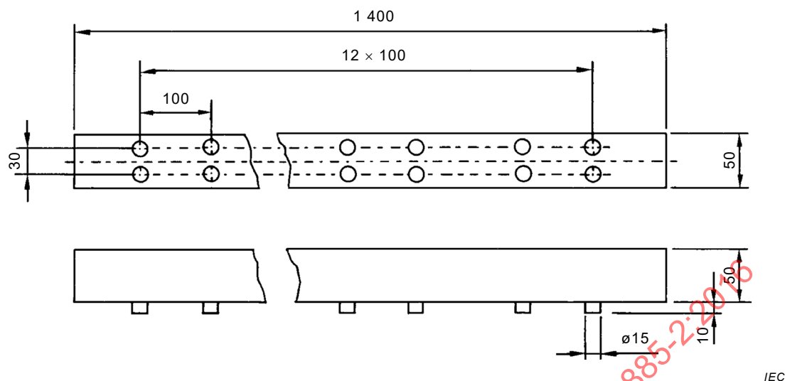
Figure 20 – Carpet hold-downs and guides
