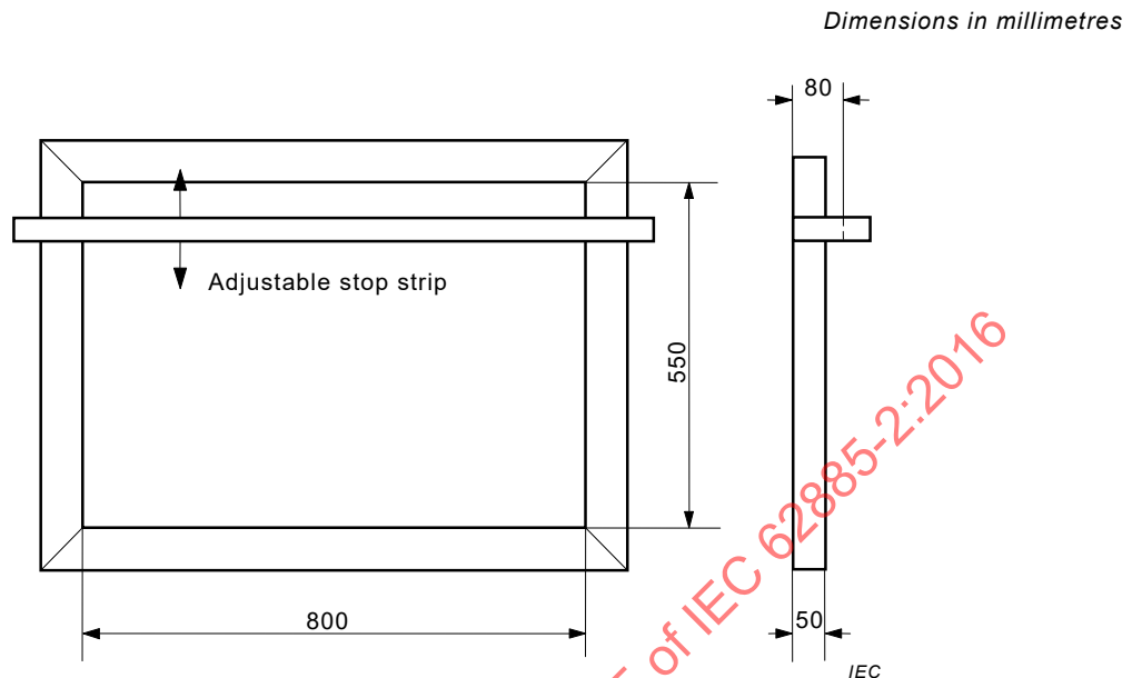
Figure 5 – Frame for test cushion
