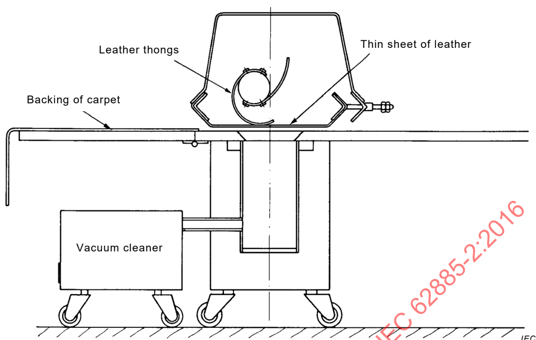
Figure 19 – Carpet-beating machine
