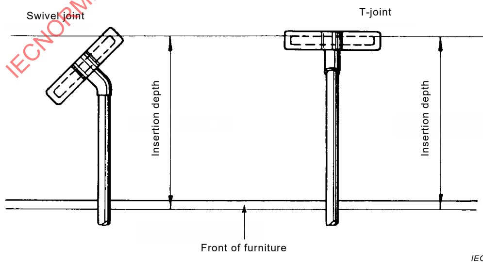
Figure 12 – Insertion depth
