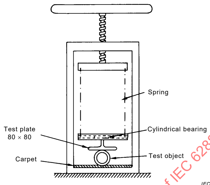
Figure 29 – Device for testing deformation of hoses and connecting tubes
