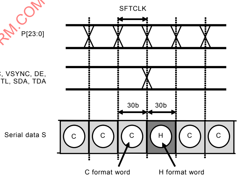
Figure 6 – Encoder output diagram
