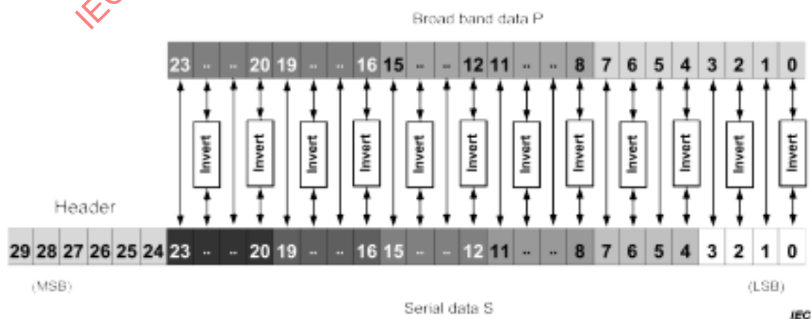
Figure 8 – H format word
