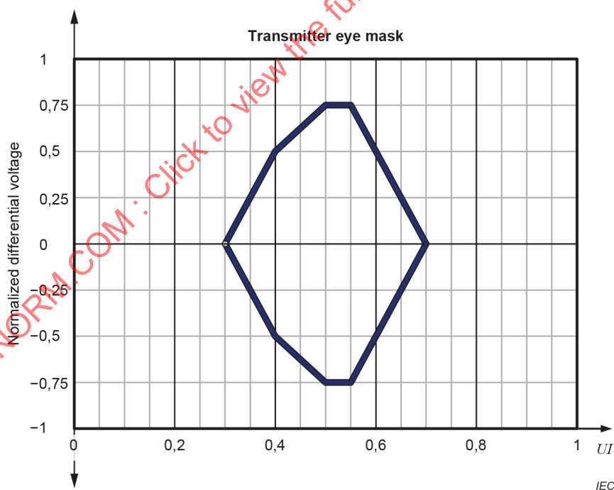
Figure B.3 – Transmitter eye mask specifications (TP1)
