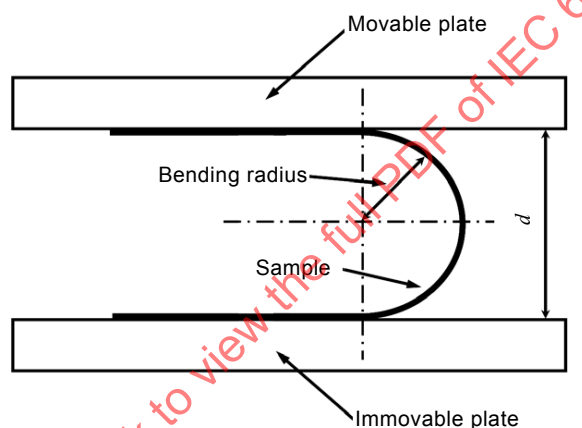
Figure 3 – Structure of the flex resistance tester near the part where the specimen is attached
