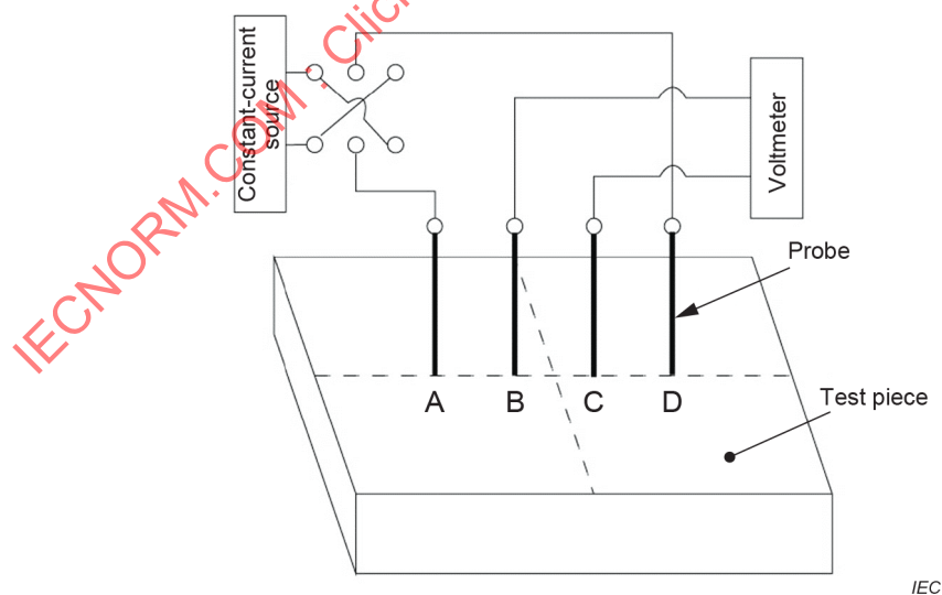
Figure 2 – Example of four-probe measurement equipment
