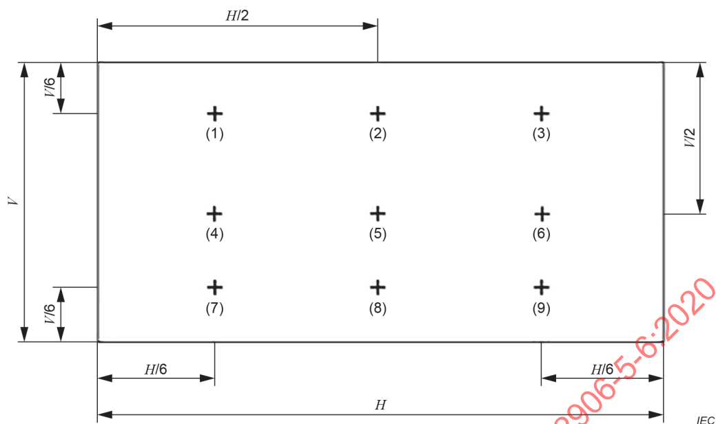
Figure 3 – Standard measurement locations on the screen (nine measurement points)
