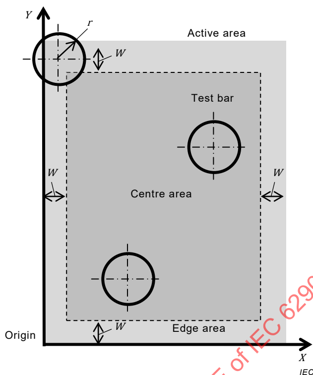
Figure 5 – Location of edge area and centre area
