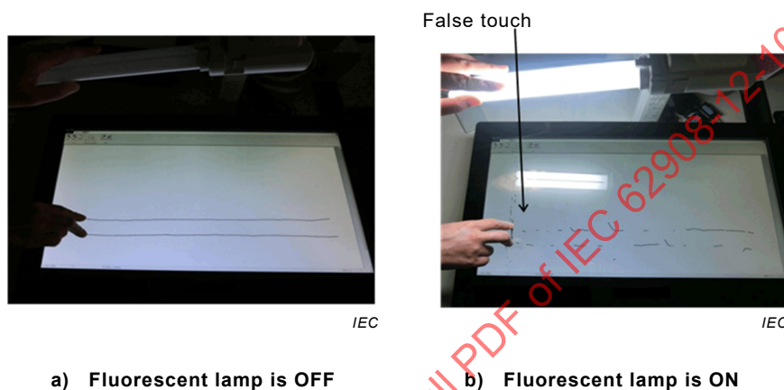
Figure 21 – Example of the effect of external noise
