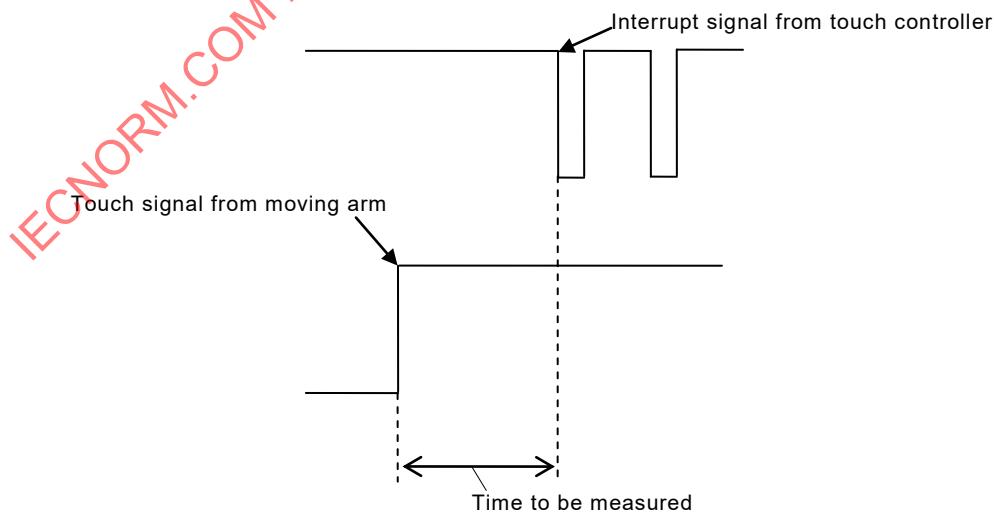
Figure 20 – Latency measurement
