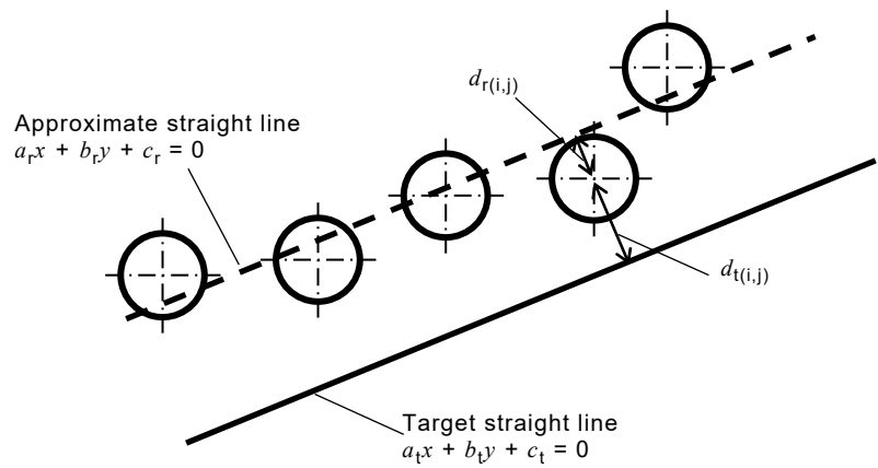
Figure 12 – Linearity definition
