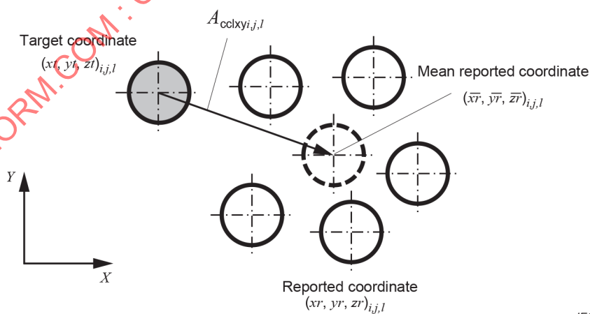
Figure 28 – Accuracy definition for in-plane of XY coordinates on the target projection plane ( l ) of the active area
