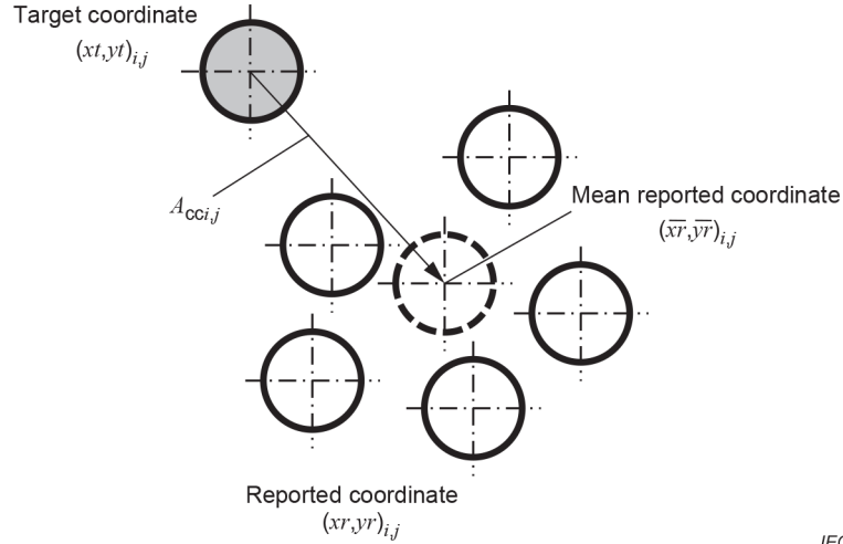
Figure 7 – Accuracy definition
