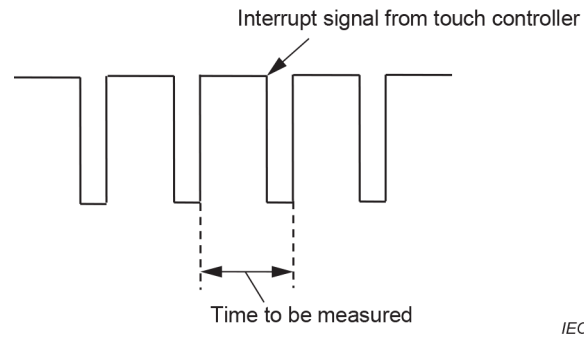
Figure 34 – Reporting time interval measurement
