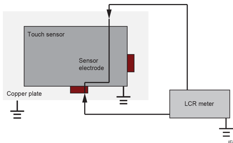
Figure A.1 – Diagrammatic representation of measurement of resistance
