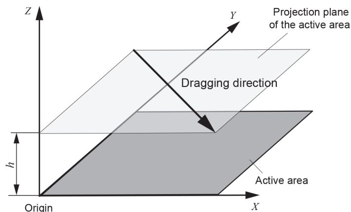
Figure 32 – Dragging direction of in-plane for reporting time measurement
