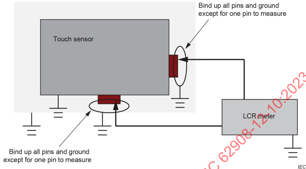
Figure A.2 – Diagrammatic representation of measurement of capacitance
