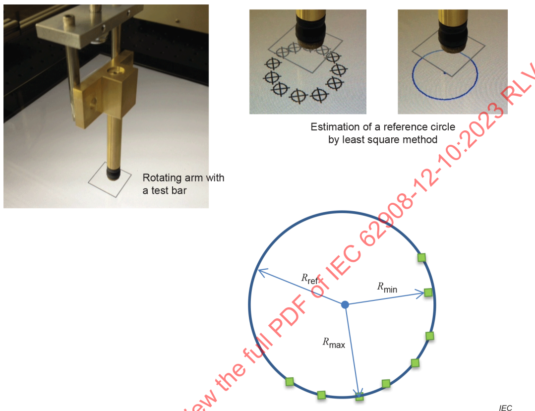
Figure 15 – Reproducibility test procedure
