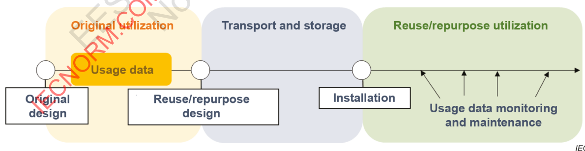
Figure 3 – Life cycle of reused or repurposed battery
