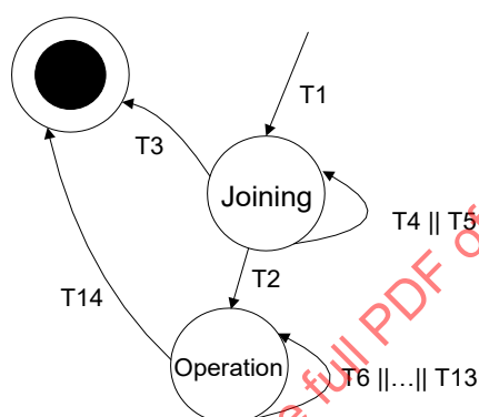
Figure 15 – DMAP state machine of an access device
