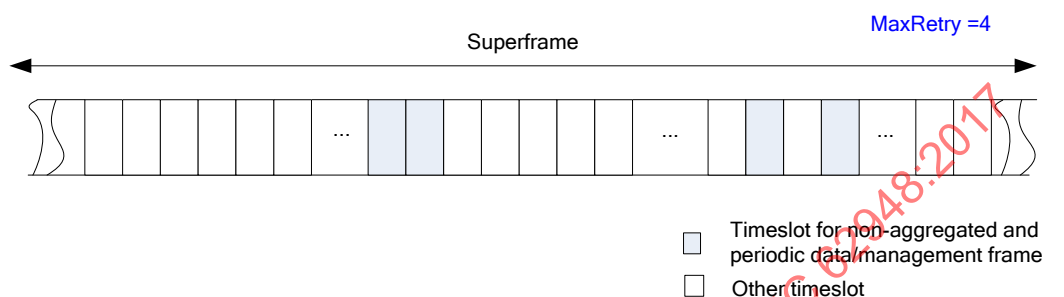
Figure 33 – Example of multi-unicast retransmission mode
