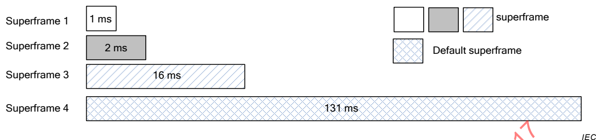
Figure 26 – WIA-FA superframe
