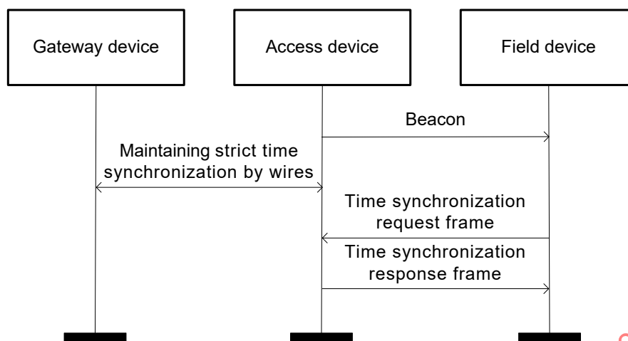
Figure 30 – Process of two-way time synchronization
