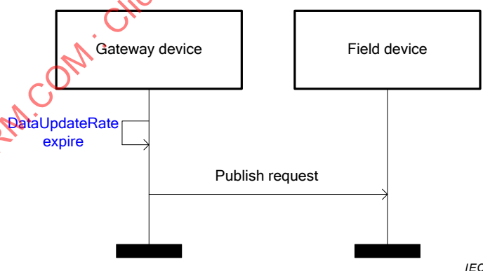
Figure 91 – Publish process from GW to FD
