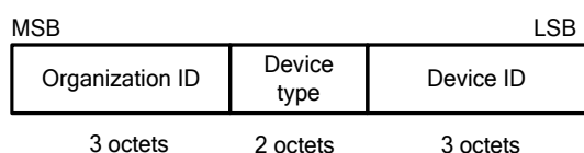
Figure 16 – Long address structure of device
