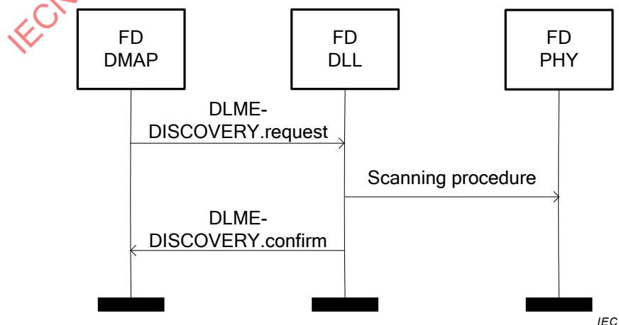
Figure 39 – Network discovery process
