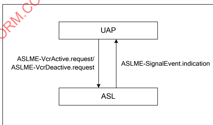
Figure 104 – ASL management service primitives between ASL and UAP
