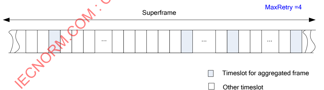
Figure 34 – Example of multi-broadcast retransmission mode
