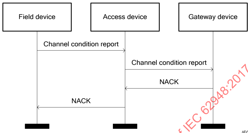
Figure 21 – Channel condition report process of field device
