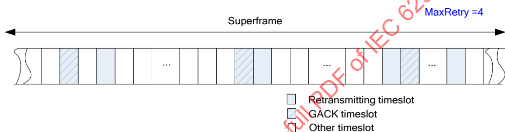
Figure 35 – Example of GACK-based timeslot backoff mode
