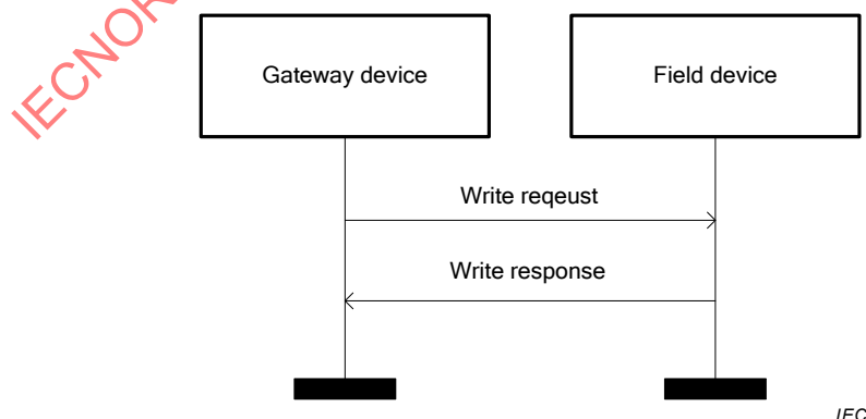
Figure 88 – Write service process
