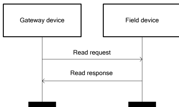
Figure 85 – Read service process
