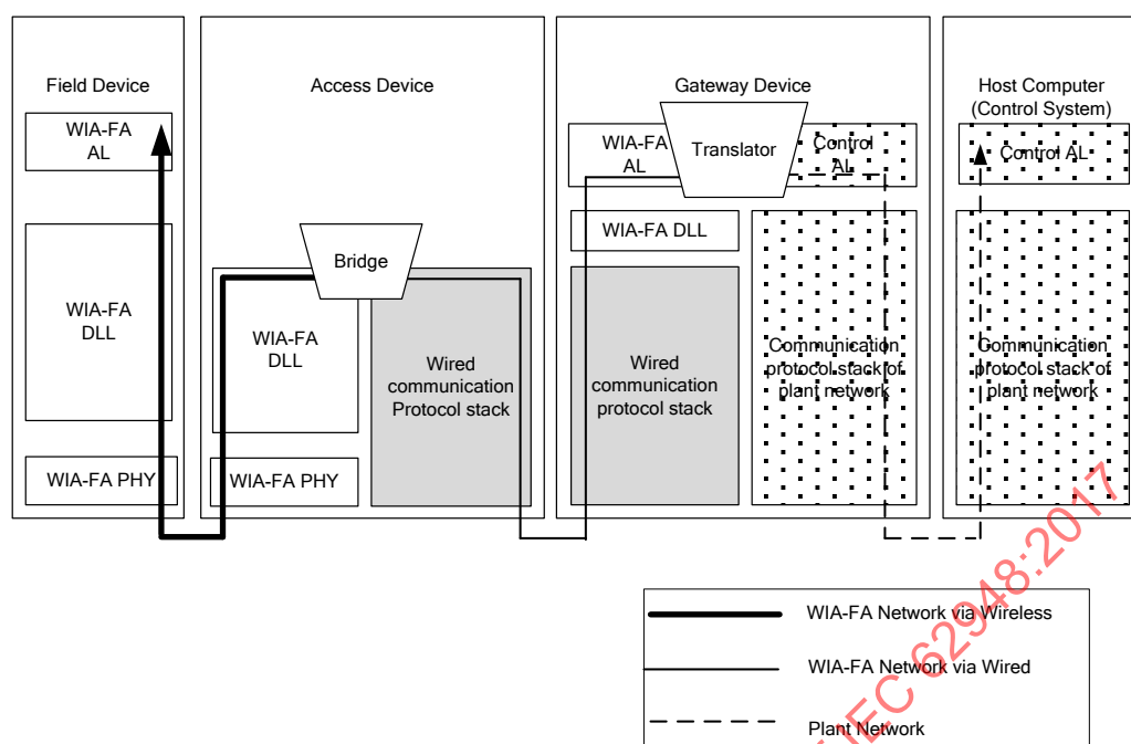
Figure 9 – Data flow over WIA-FA network
