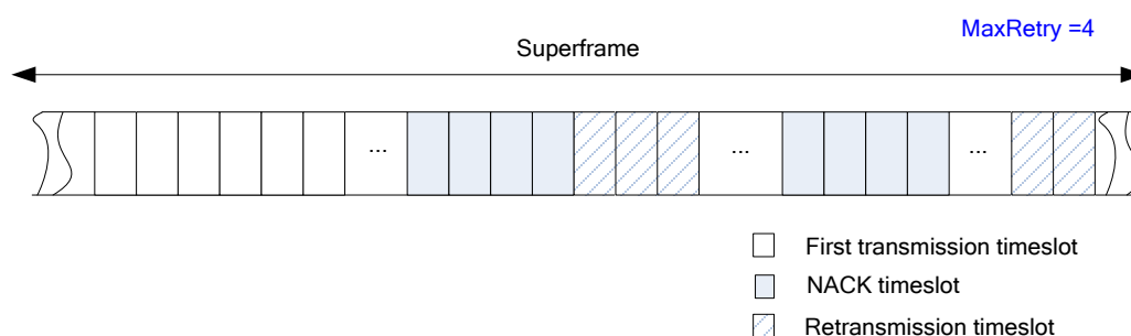
Figure 32 – Example of NACK-based retransmission mode
