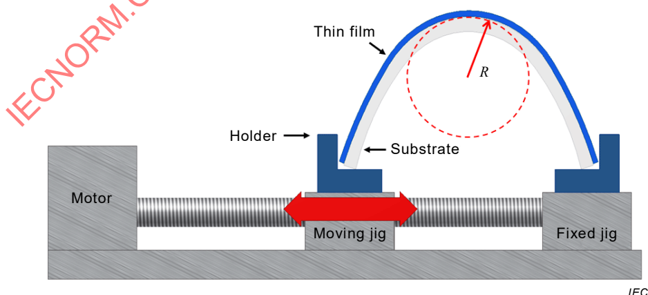
Figure 2 – Bending test apparatus
