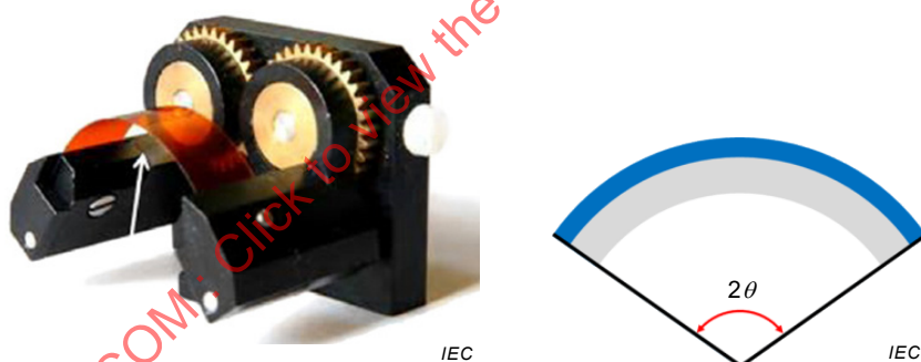
Figure A.1 – X-Y- \theta bending test method
