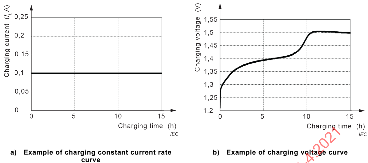
Figure A.2 – Examples of Ni-MH charge curves
