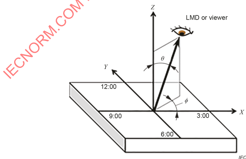
Figure 1 – Cartesian coordinate system and spherical coordinate system for the specification of the viewer's gazing (viewing) direction
