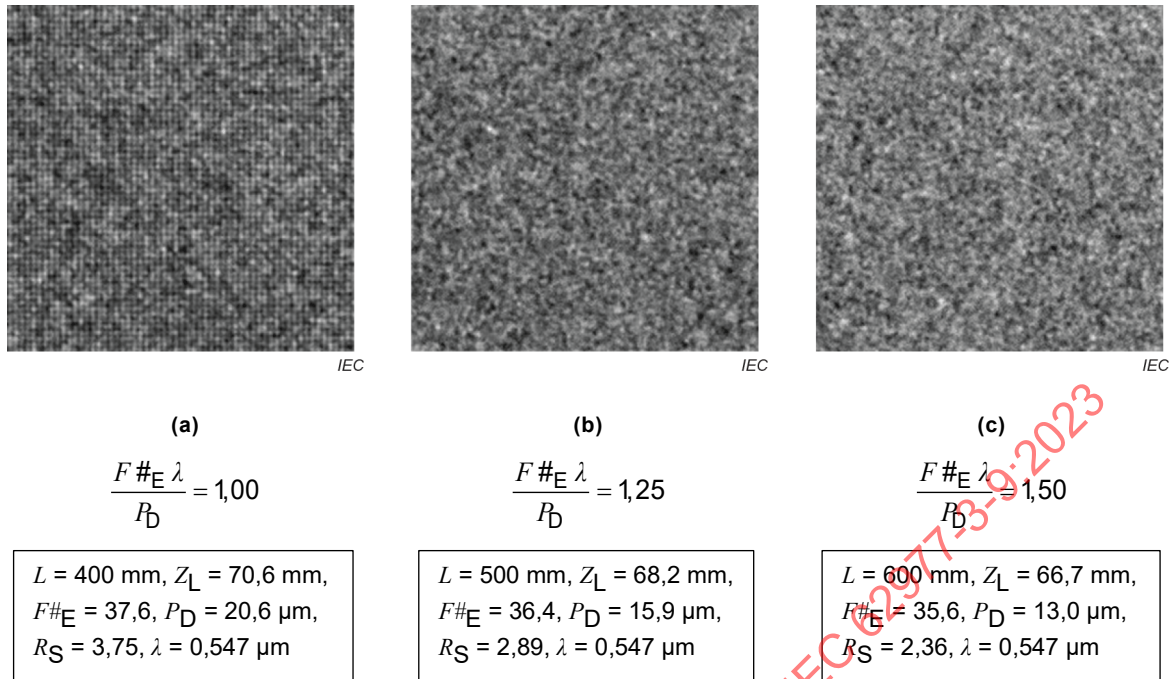
Figure A.1 – Examples of sparkle image from the same DUT under different measurement distances
