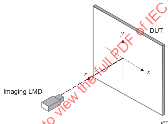
Figure 3 – Measurement setup
