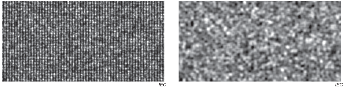
Figure B.2 – Examples of sparkle patterns at R_S = 4,3 before applying an MWA filter (left) and after applying an MWA filter (right)
