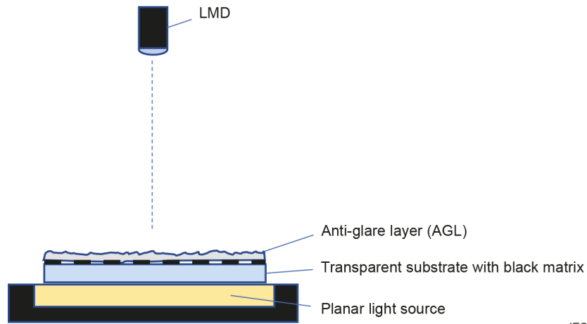
Figure D.2 – Example of measurement configuration
