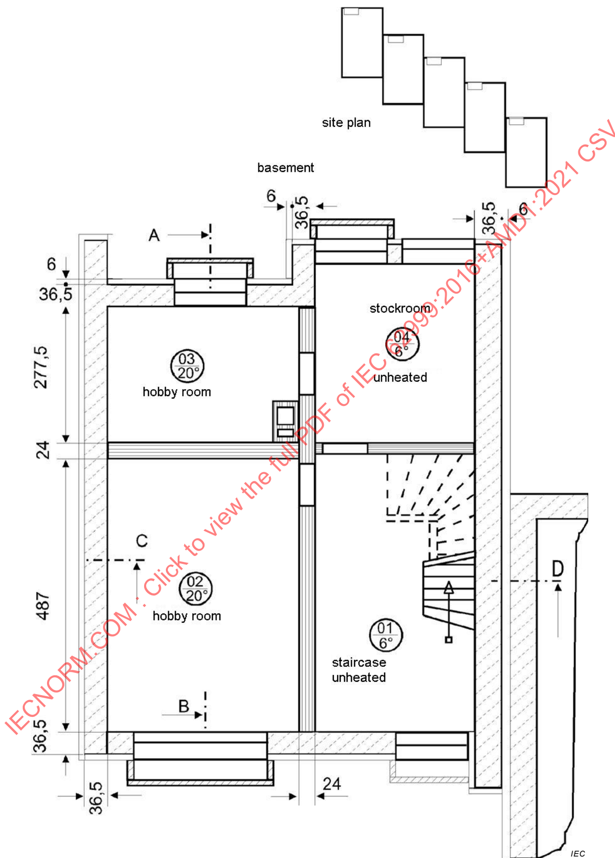
Figure A.4 – Plan of basement
