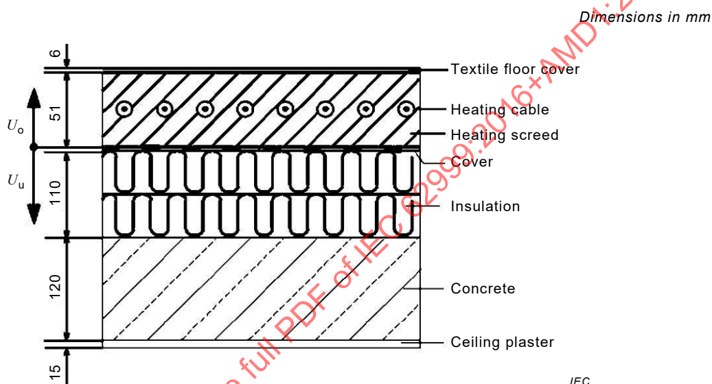
Figure C.1 – Ceiling construction
