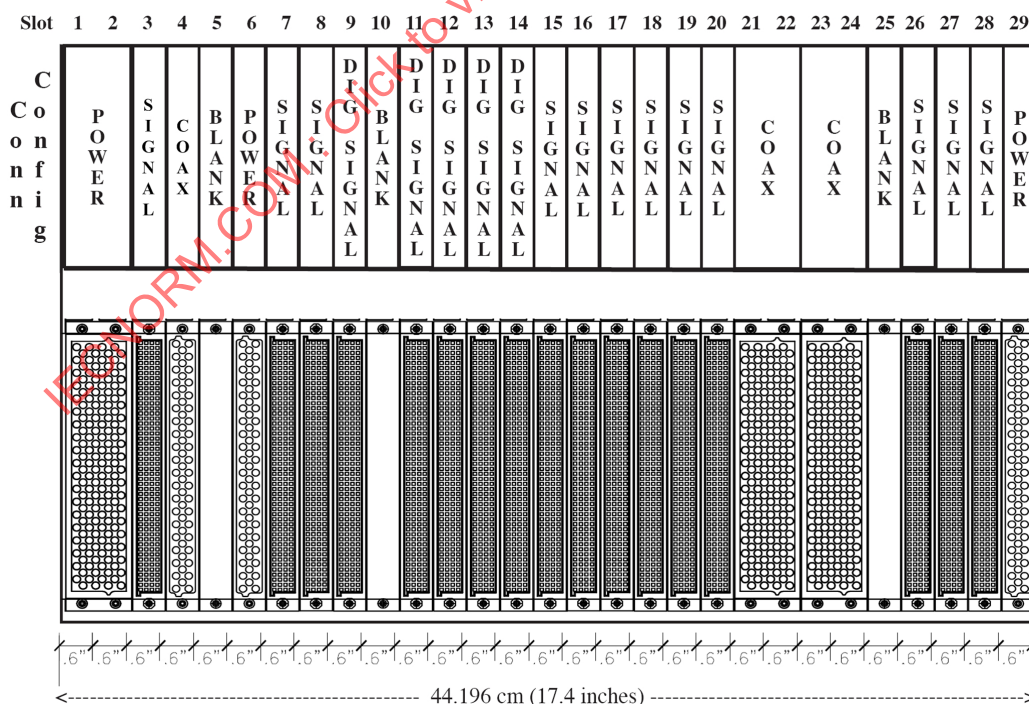
Figure 2—CTI system 29-slot receiver connector configuration
