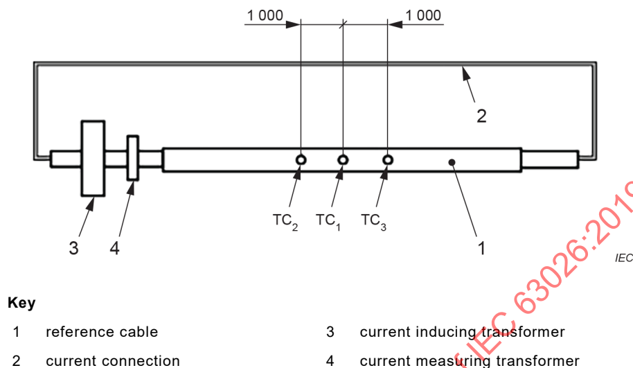
Figure A.5 – Reference cable for heating of single-core armoured cables
