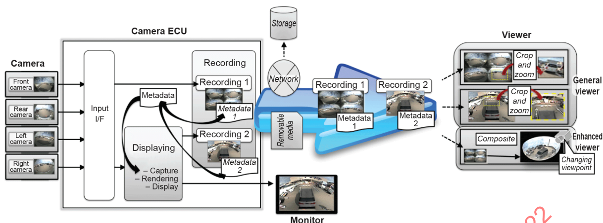
Figure 1 – Display and recording system model of surround view system
