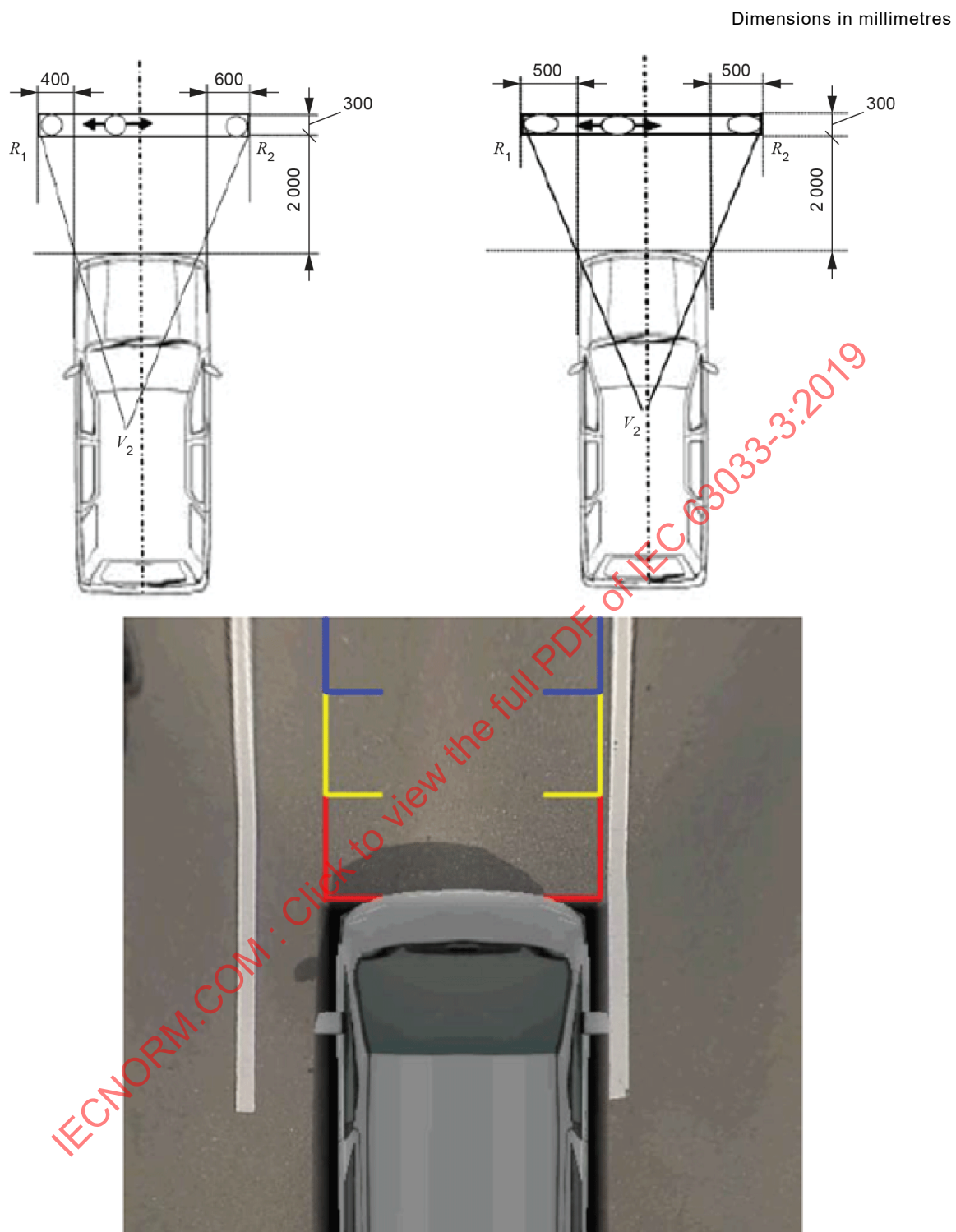
Figure A.8 – Example view for FOV of 5.4.1 defined in UN Regulation No. 125
