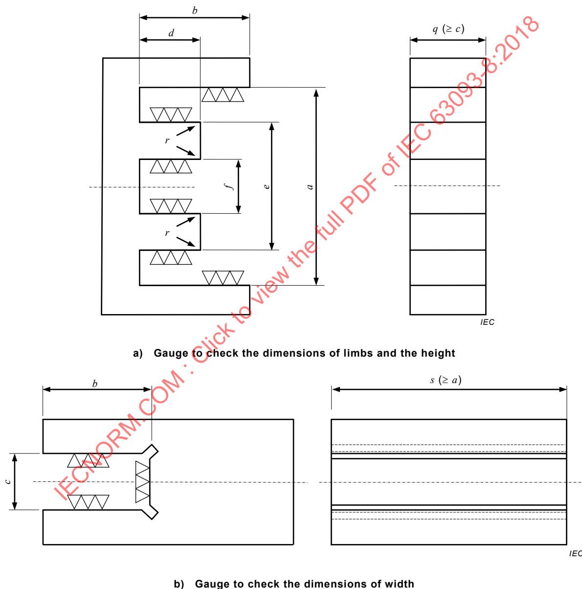
Figure B.1 – Gauge dimensions
