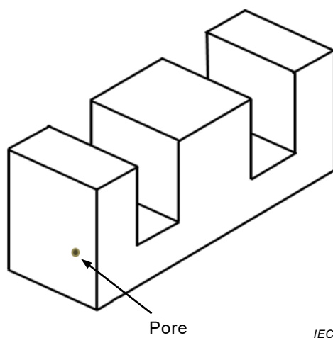
Figure 7 – Pore location for E-cores
