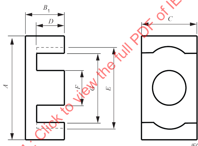
Figure 15 – Reference dimensions for ER-core
