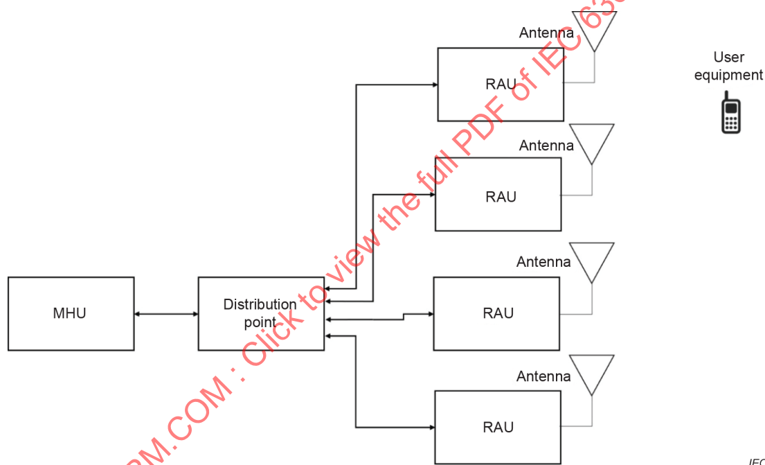
Figure 3 – Point-to-multipoint configuration of DAS
