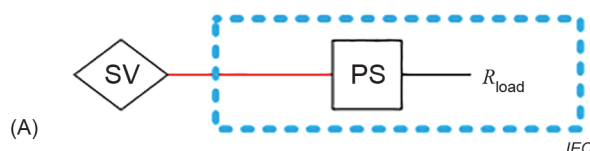
Figure B.2 – Measurement setup for determining the input power supplied to the power supply
