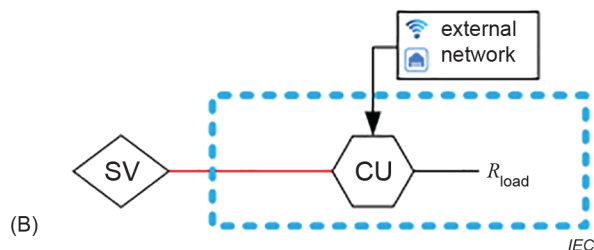
Figure B.3 – Measurement setup (with optional network provision) for determining the input power supplied to the control unit
