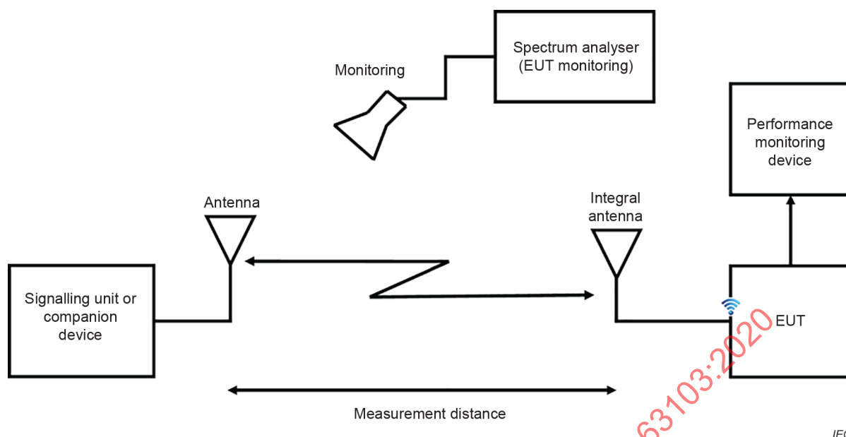
Figure 2 – Test setup for non-active mode power consumption measurement of connected EUT with integral antennas (RF path symbolically shown)
