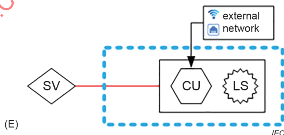
Figure B.6 – Measurement setup (with optional network provision) for determining the input power supplied to the combined light source and control unit
