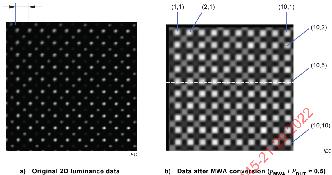
Figure A.2 – Example of MWA conversion of 2D luminance data (image)
