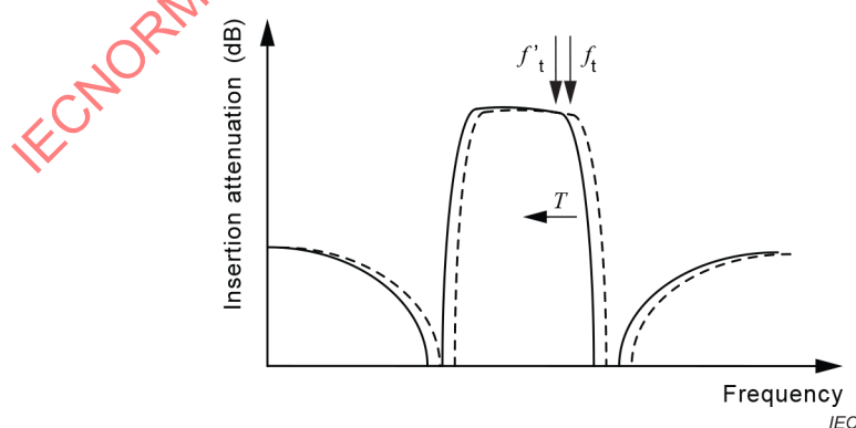
Figure 8 – Translation of the filter pass band with temperature change
