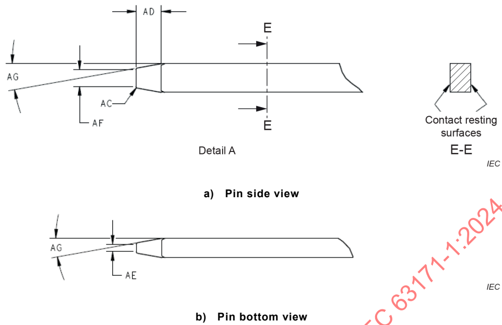
Figure 5 – Fixed Type 1 connector pin detail (detail A from Figure 4c) section D-D)
