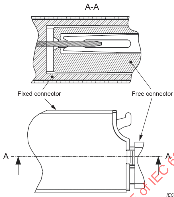
Figure 3 – Mated fixed and free Type 1 connectors
