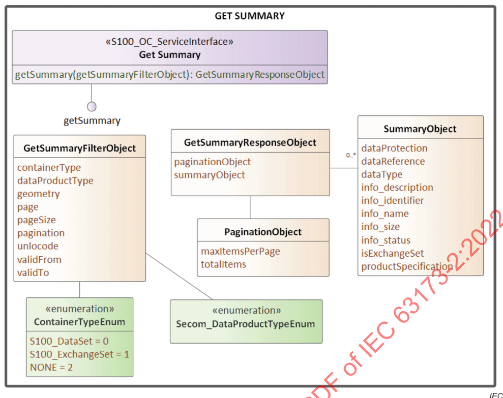
Figure 20 – Diagramme UML de l'interface Get Summary
