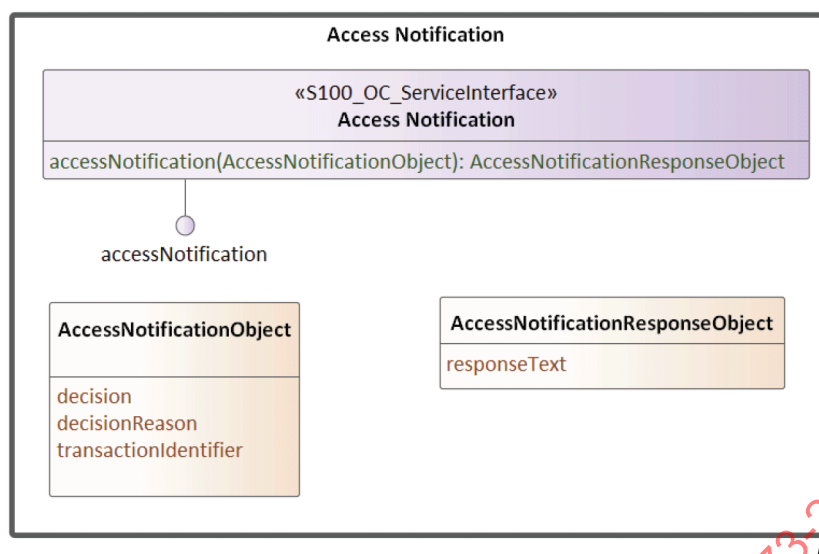
Figure 26 – Diagramme UML de l'interface Access Notification
