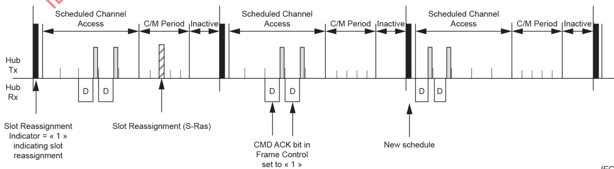
Figure 19 – Slot reassignment illustration
