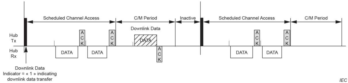
Figure 18 – Downlink data transmission illustration
